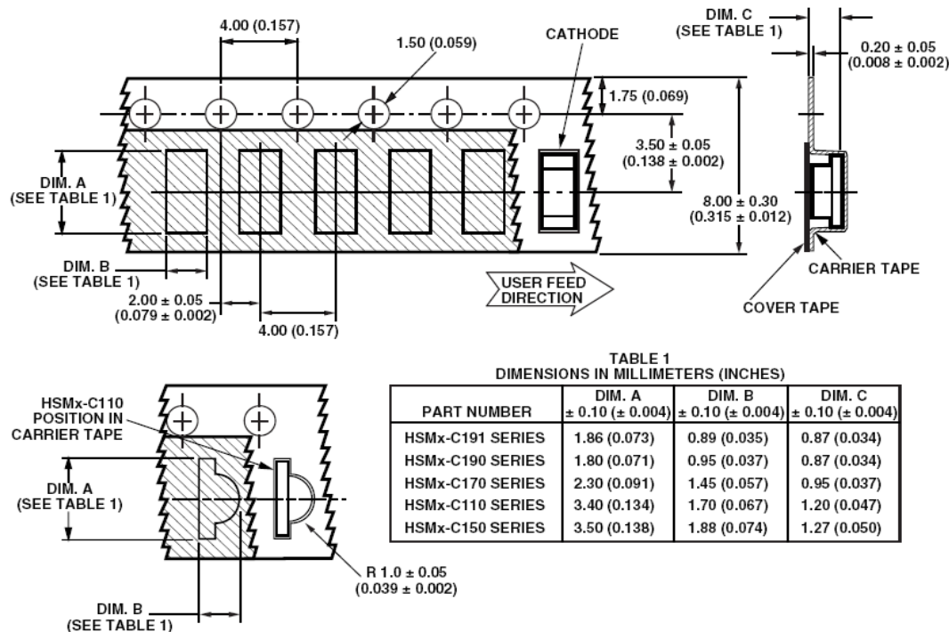
Figure 15. Tape dimensions.
