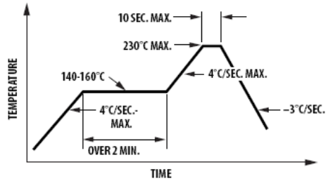
Figure 7. Recommended reflow soldering profile.
