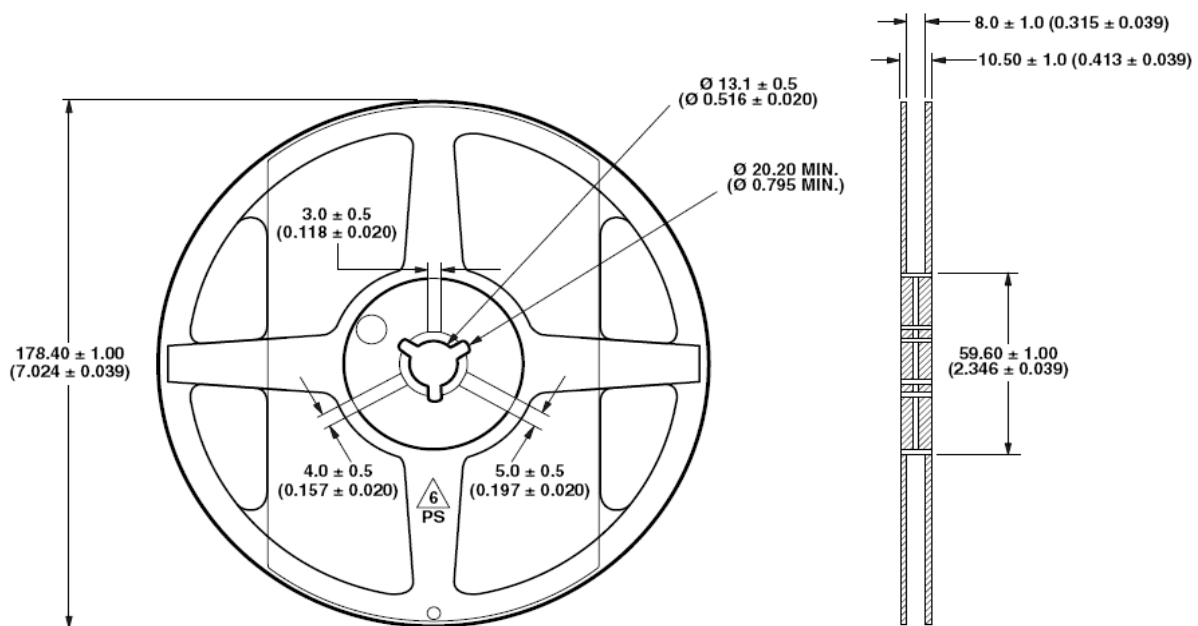
Figure 14. Reel dimensions.
